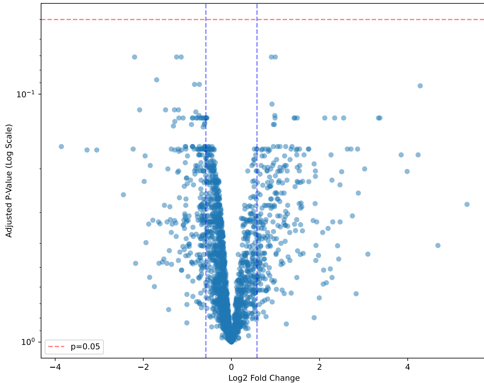
Volcano Plot: D7 - T0
